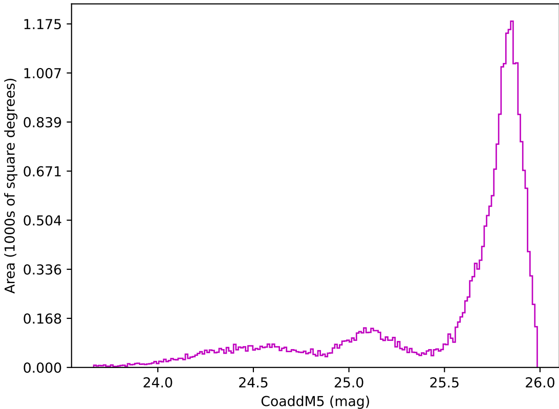
weather_cloudso18v3.4_10yrs All sky z band: CoaddM5
