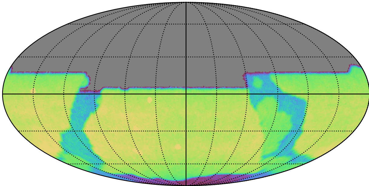
weather_cloudso18v3.4_10yrs All sky y band: CoaddM5
