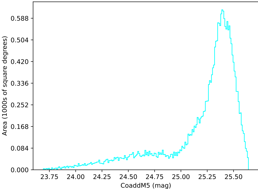
weather_cloudso18v3.4_10yrs All sky u band: CoaddM5
