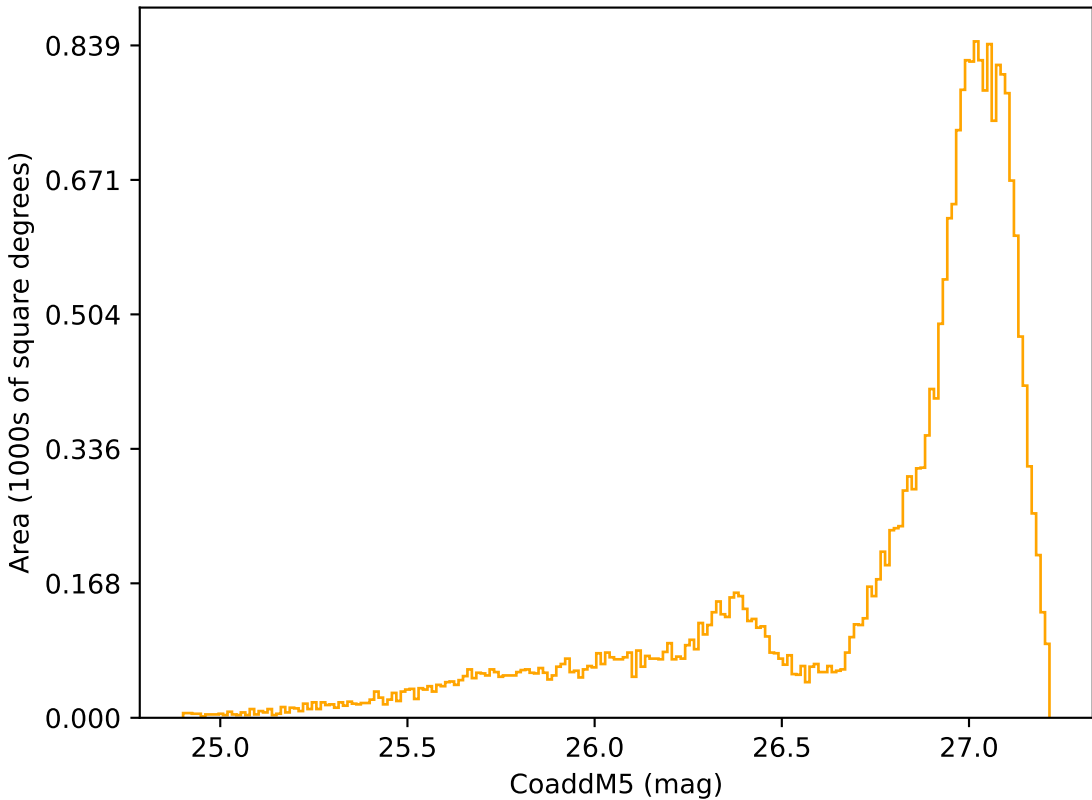
weather_cloudso18v3.4_10yrs All sky r band: CoaddM5
