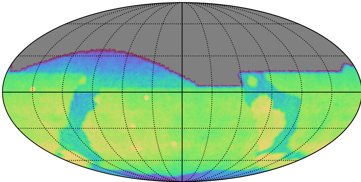
weather_cloudso18v3.4_10yrs All sky g band: CoaddM5
