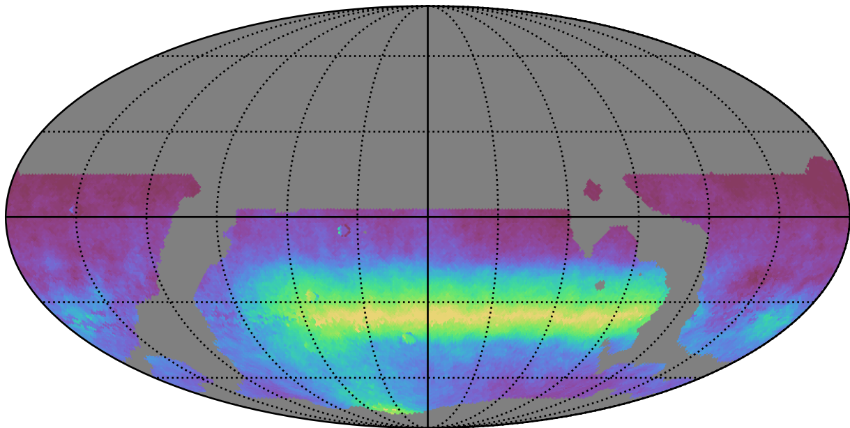
weather_cloudso18v3.4_10yrs WFD all bands: AngleRms rotSkyPos
