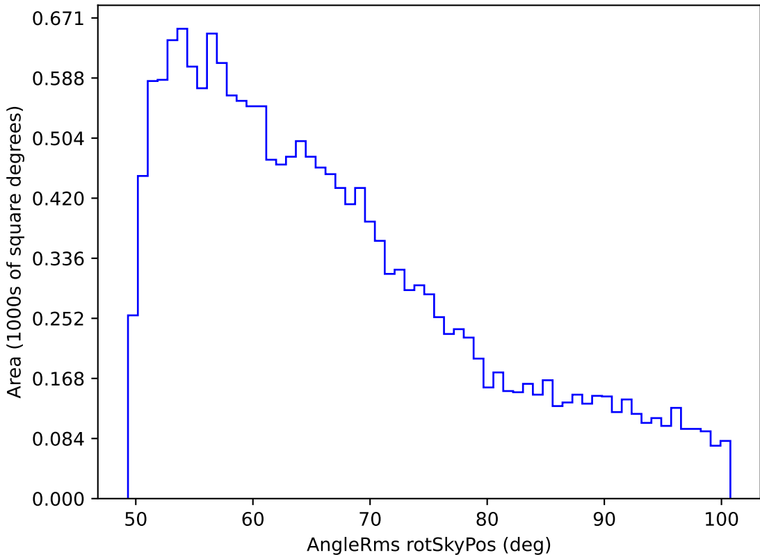
weather_cloudso18v3.4_10yrs WFD all bands: AngleRms rotSkyPos
