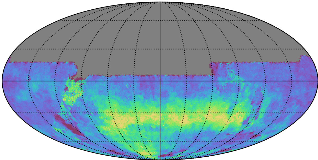
weather_cloudso18v3.4_10yrs All sky u band: AngleRms rotSkyPos
