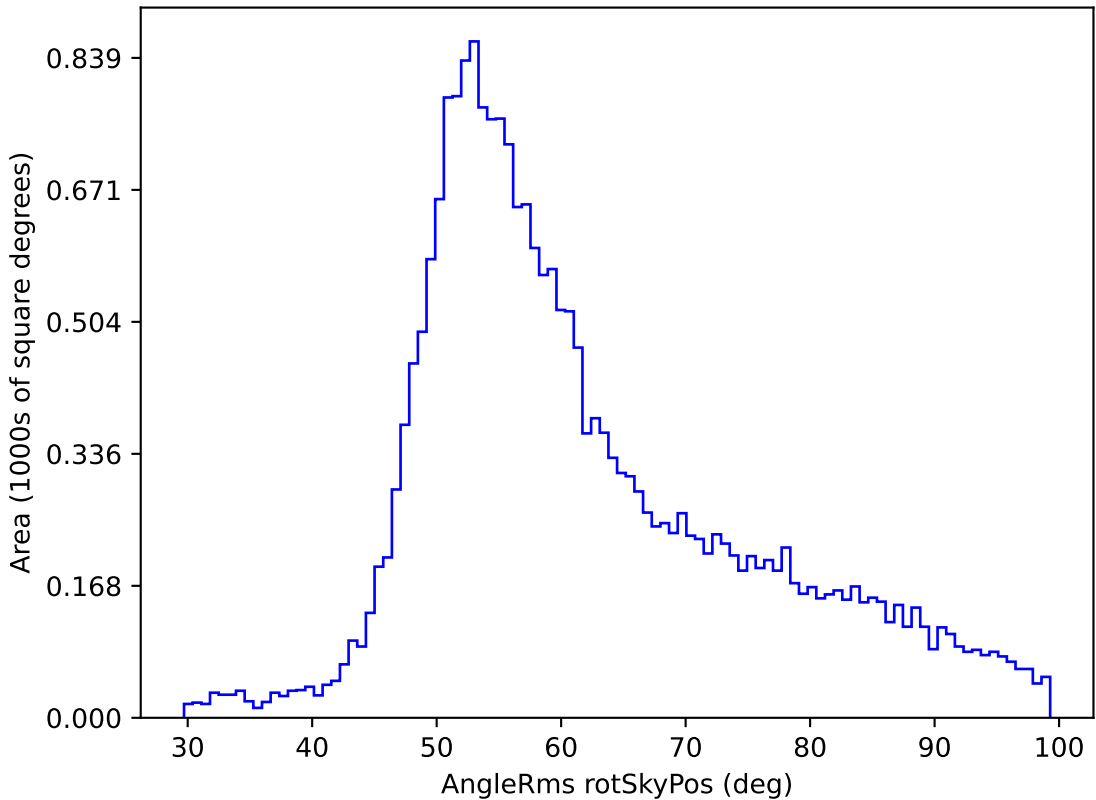
weather_cloudso18v3.4_10yrs All sky u band: AngleRms rotSkyPos
