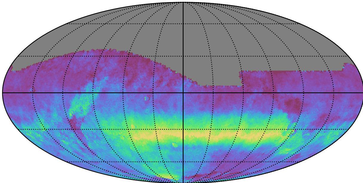
weather_cloudso18v3.4_10yrs All sky r band: AngleRms rotSkyPos
