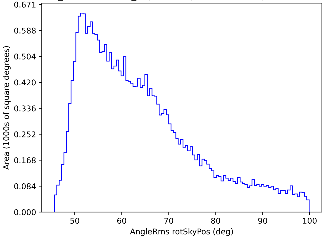
weather_cloudso18v3.4_10yrs All sky all bands: AngleRms rotSkyPos
