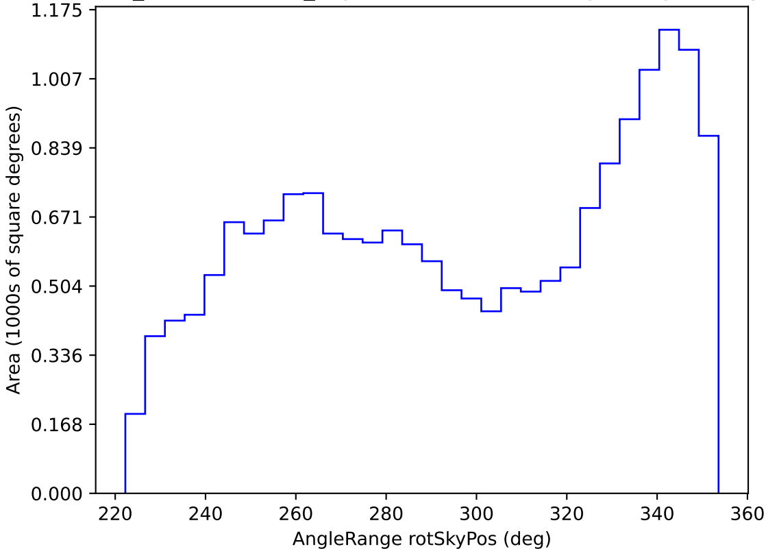
weather_cloudso18v3.4_10yrs WFD all bands: AngleRange rotSkyPos
