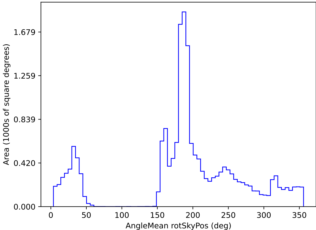
weather_cloudso18v3.4_10yrs WFD all bands: AngleMean rotSkyPos
