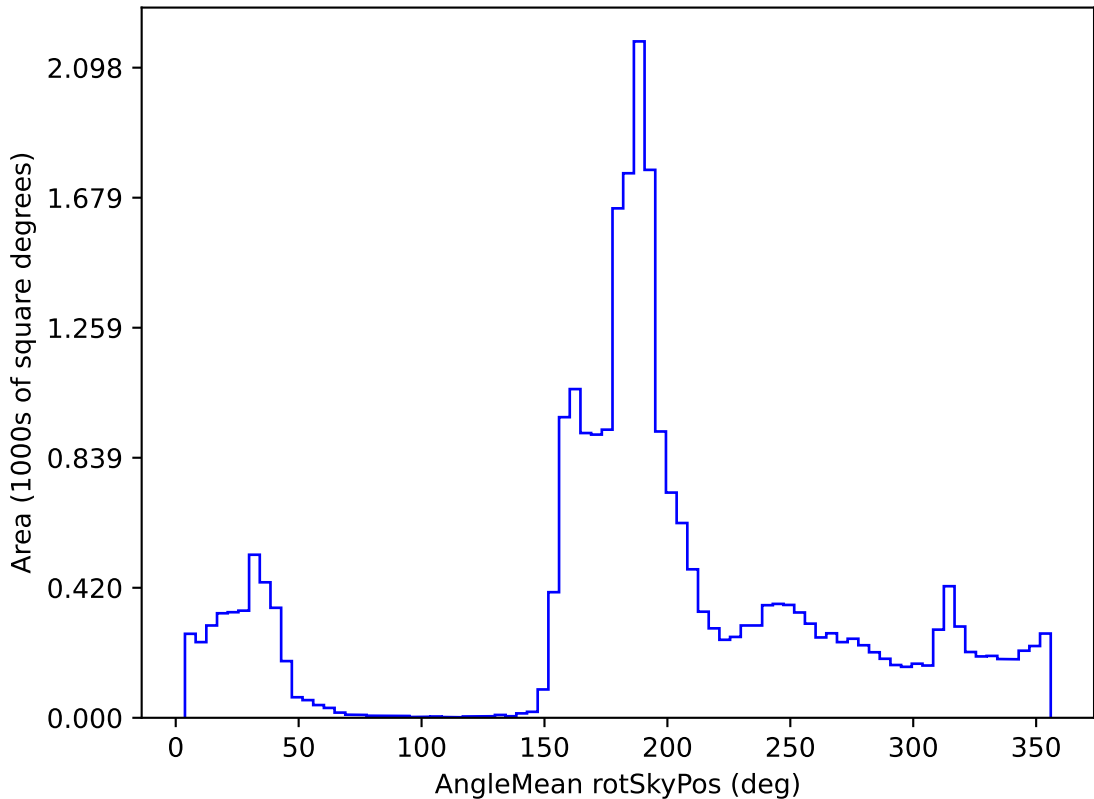
weather_cloudso18v3.4_10yrs All sky all bands: AngleMean rotSkyPos
