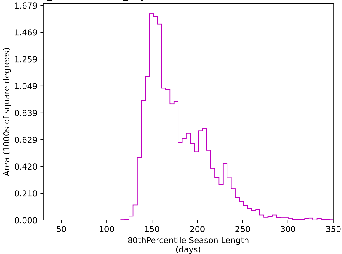
weather_cloudso18v3.4_10yrs WFD z band: 80thPercentile Season Length
