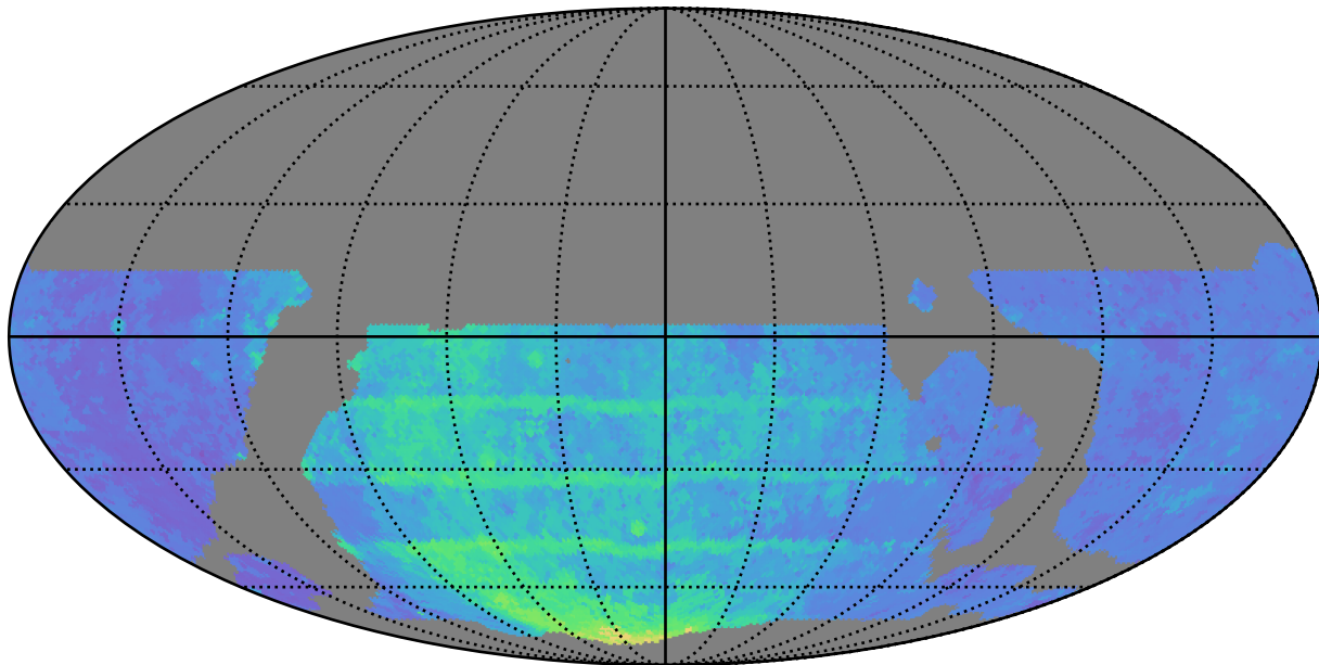
weather_cloudso18v3.4_10yrs WFD y band: 80thPercentile Season Length
