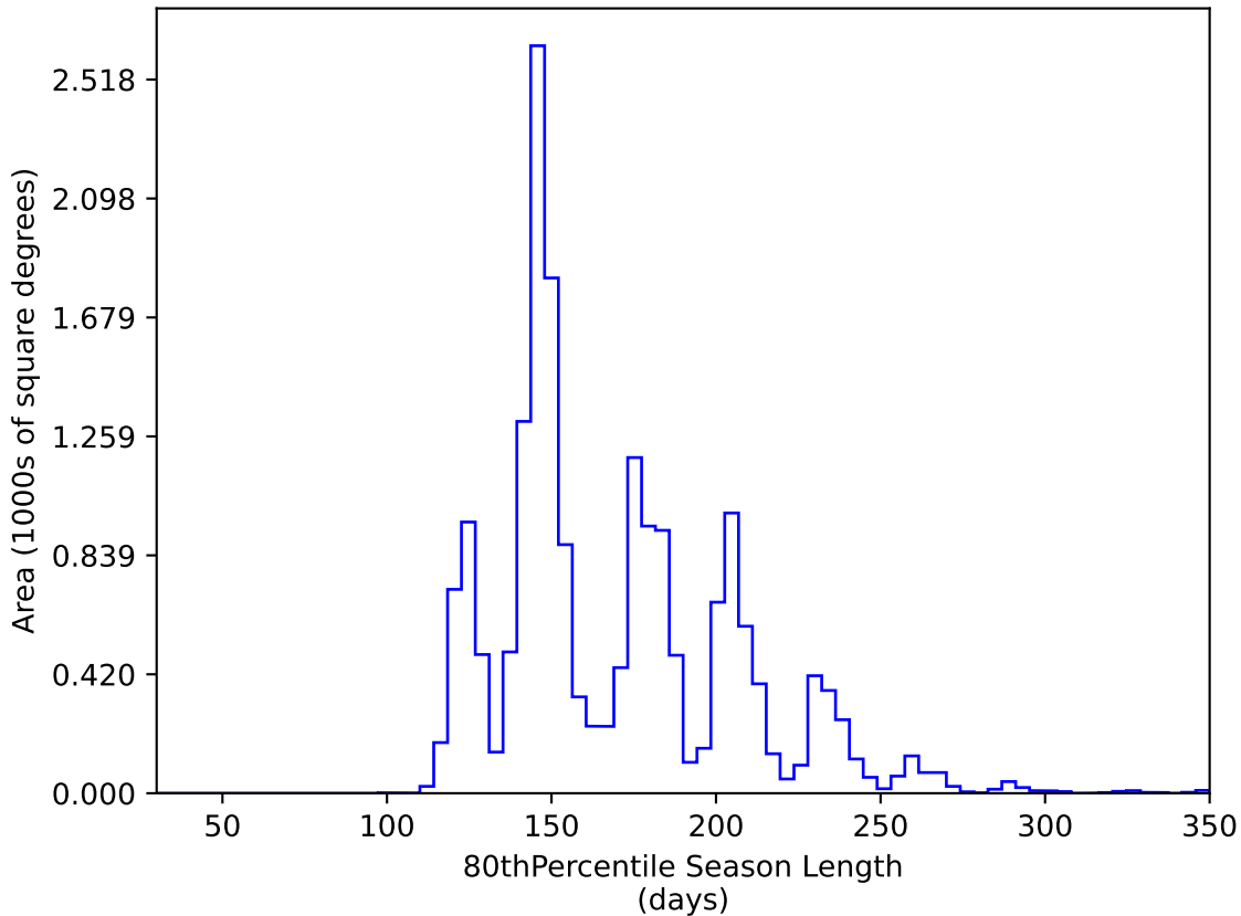
weather_cloudso18v3.4_10yrs WFD y band: 80thPercentile Season Length
