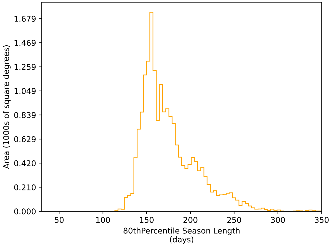
weather_cloudso18v3.4_10yrs WFD r band: 80thPercentile Season Length
