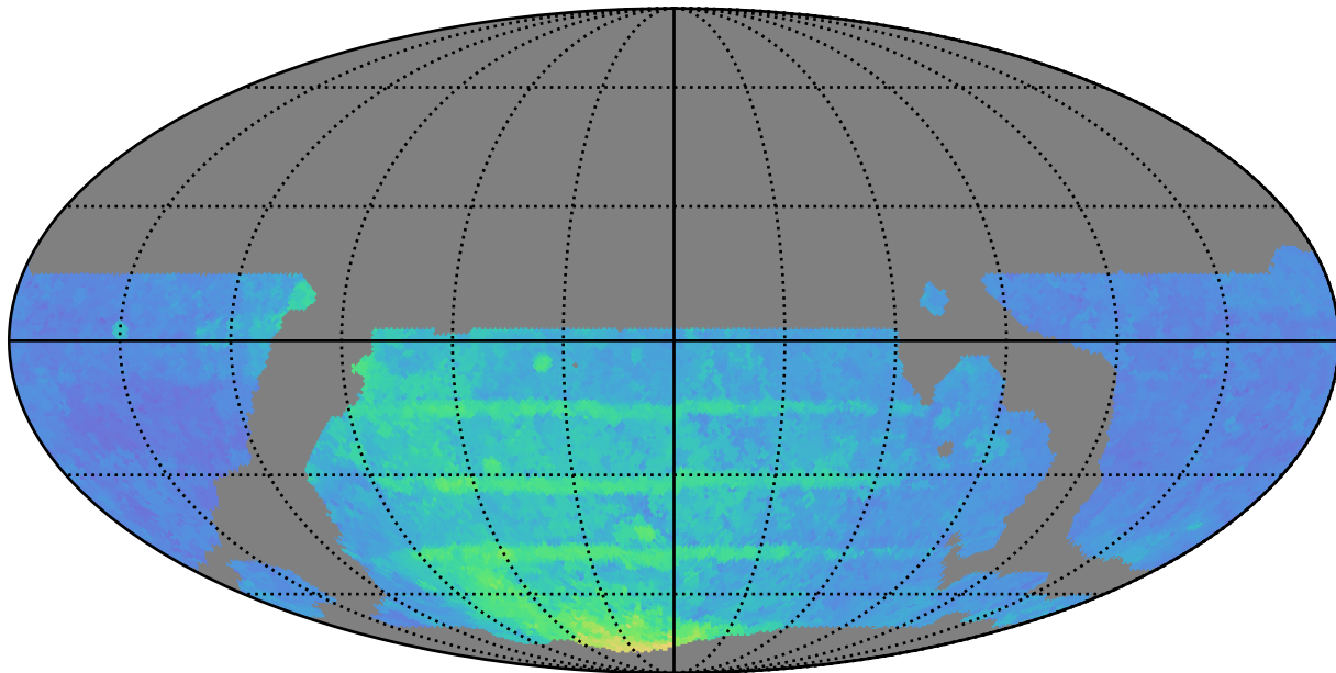
weather_cloudso18v3.4_10yrs WFD i band: 80thPercentile Season Length
