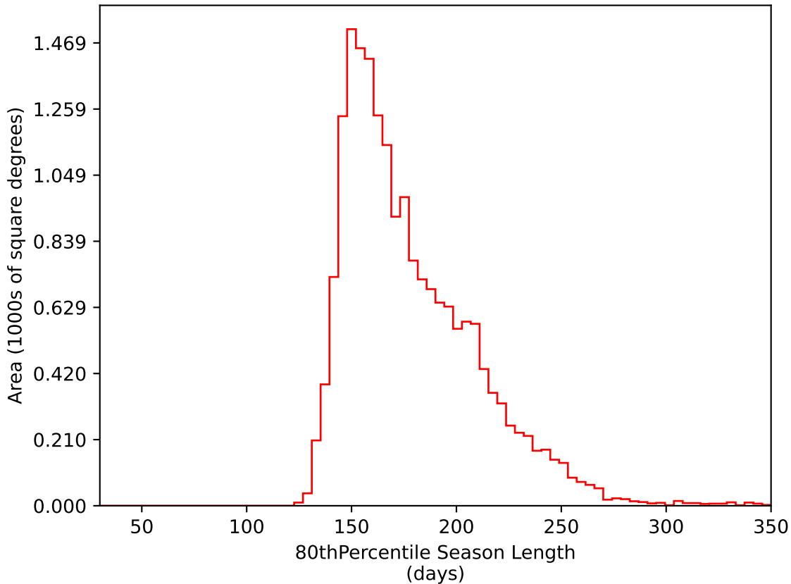
weather_cloudso18v3.4_10yrs WFD i band: 80thPercentile Season Length
