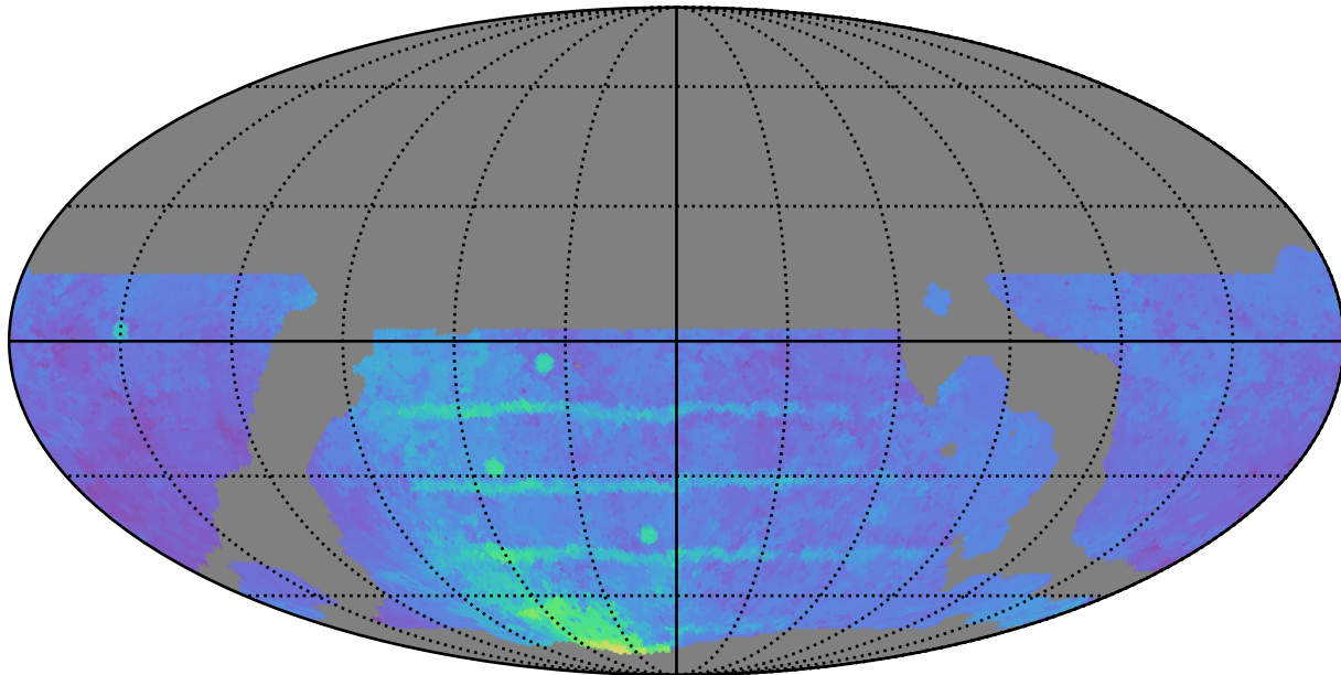
weather_cloudso18v3.4_10yrs WFD g band: 80thPercentile Season Length
