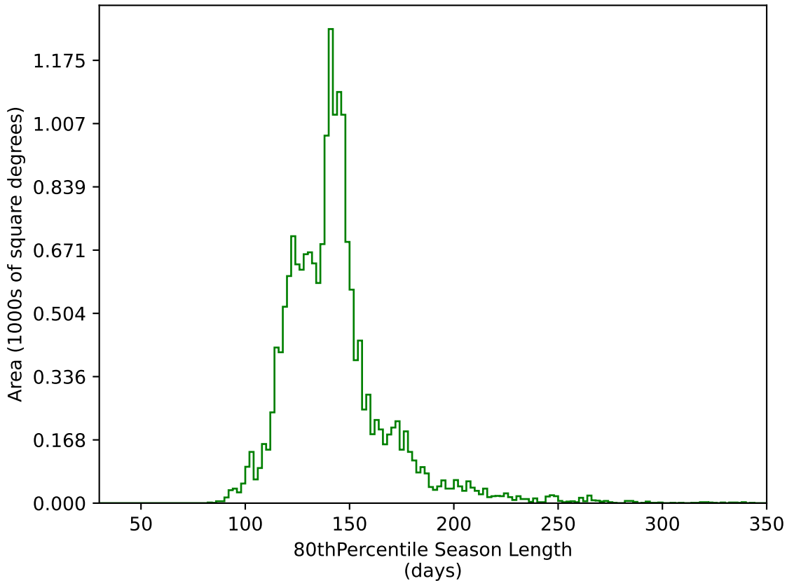
weather_cloudso18v3.4_10yrs WFD g band: 80thPercentile Season Length
