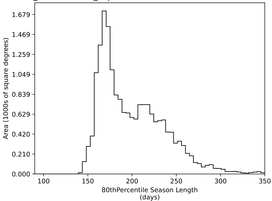
weather_cloudso18v3.4_10yrs WFD all bands: 80thPercentile Season Length
