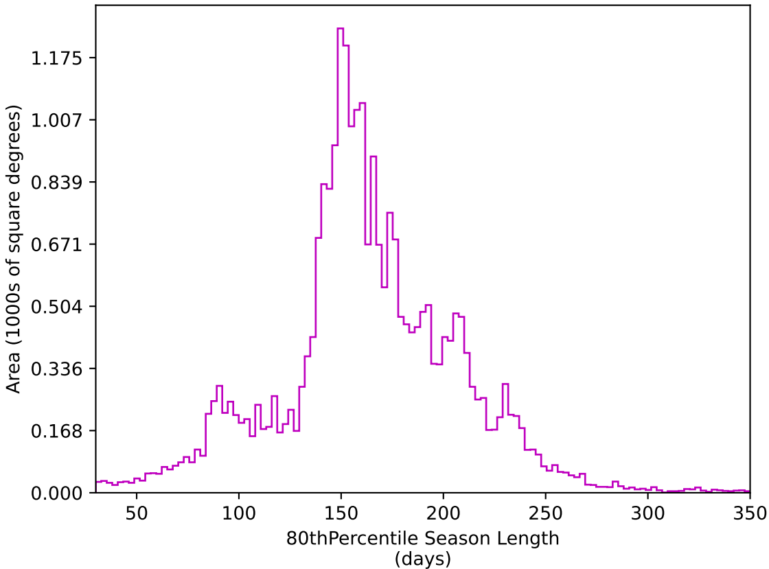
weather_cloudso18v3.4_10yrs All sky z band: 80thPercentile Season Length
