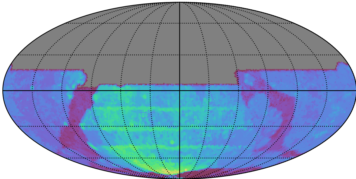
weather_cloudso18v3.4_10yrs All sky y band: 80thPercentile Season Length
