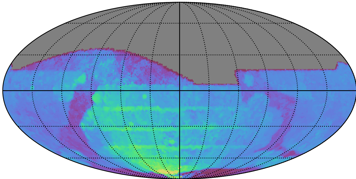
weather_cloudso18v3.4_10yrs All sky r band: 80thPercentile Season Length
