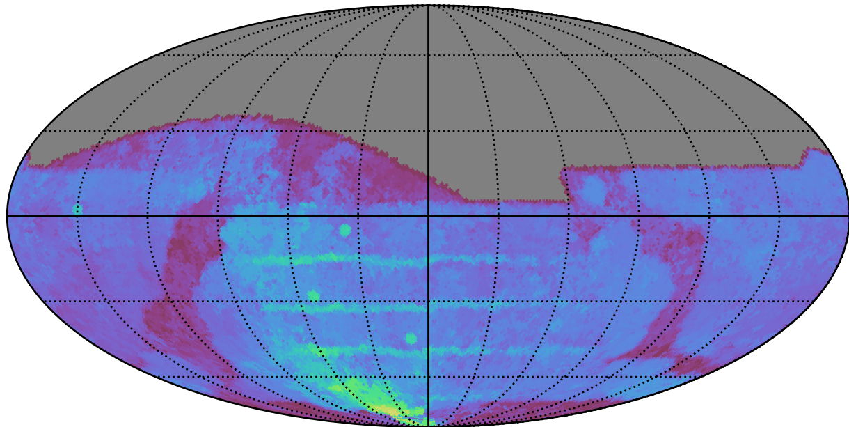
weather_cloudso18v3.4_10yrs All sky g band: 80thPercentile Season Length
