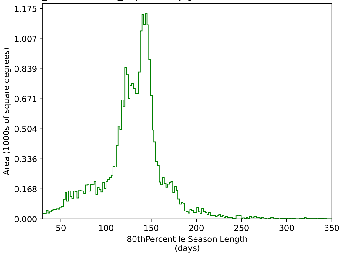
weather_cloudso18v3.4_10yrs All sky g band: 80thPercentile Season Length
