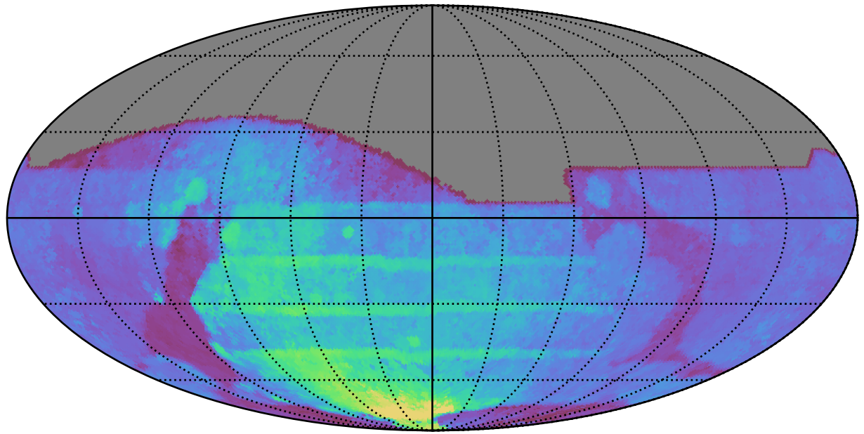
weather_cloudso18v3.4_10yrs All sky all bands: 80thPercentile Season Length
