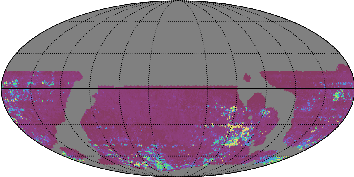
weather_cloudso18v3.4_10yrs WFD z band: 75th Percentile Intranight Timespan
