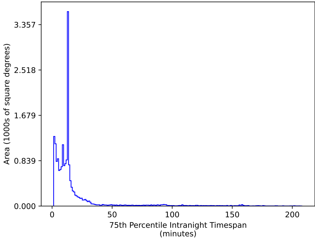
weather_cloudso18v3.4_10yrs WFD z band: 75th Percentile Intranight Timespan
