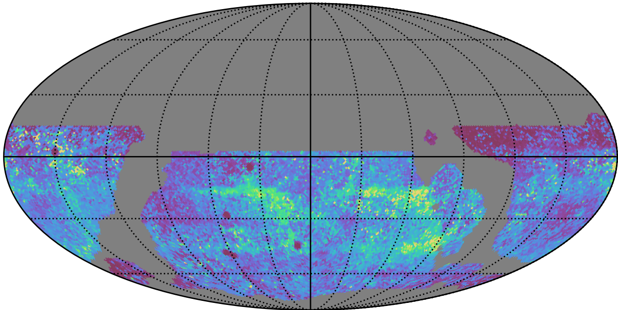
weather_cloudso18v3.4_10yrs WFD y band: 75th Percentile Intranight Timespan
