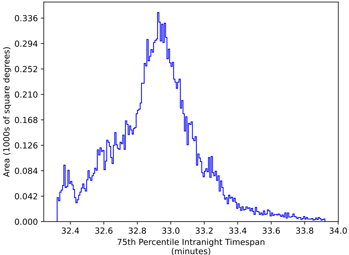
weather_cloudso18v3.4_10yrs WFD y band: 75th Percentile Intranight Timespan
