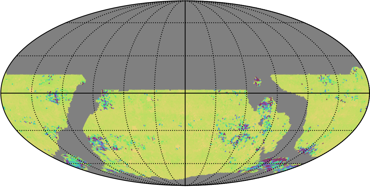
weather_cloudso18v3.4_10yrs WFD ug bands: 75th Percentile Intranight Timespan
