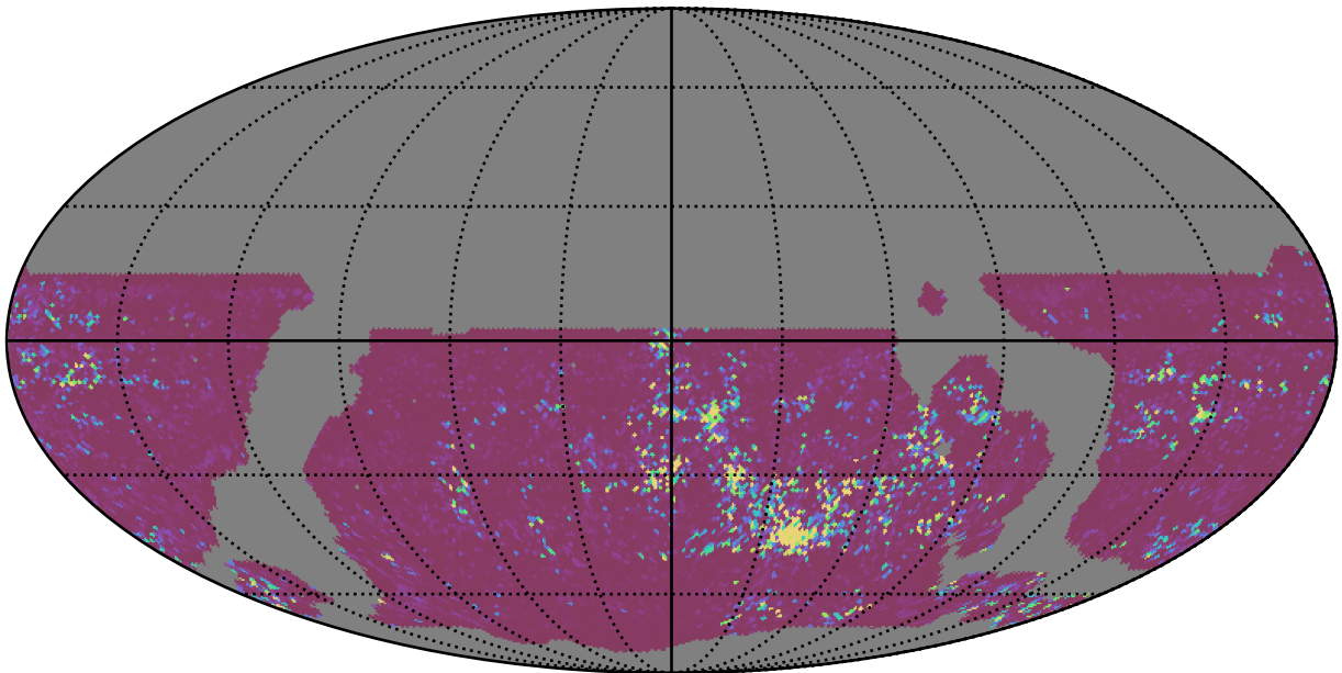
weather_cloudso18v3.4_10yrs WFD u band: 75th Percentile Intranight Timespan
