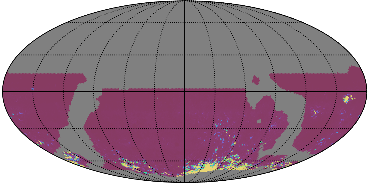
weather_cloudso18v3.4_10yrs WFD ri bands: 75th Percentile Intranight Timespan
