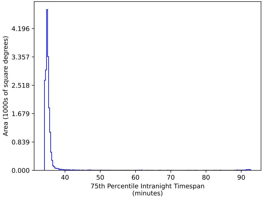
weather_cloudso18v3.4_10yrs WFD ri bands: 75th Percentile Intranight Timespan
