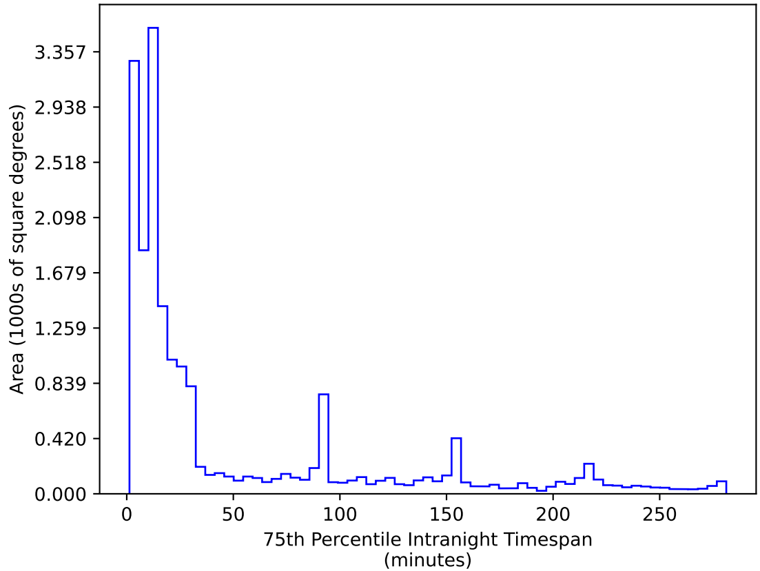
weather_cloudso18v3.4_10yrs WFD r band: 75th Percentile Intranight Timespan
