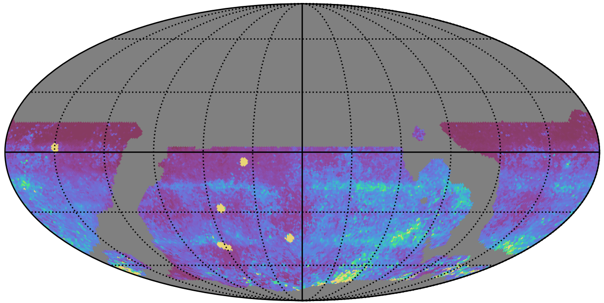
weather_cloudso18v3.4_10yrs WFD iz bands: 75th Percentile Intranight Timespan
