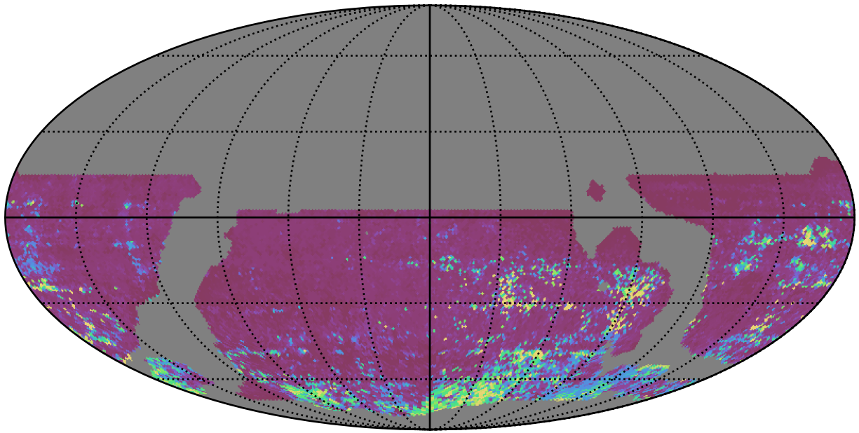
weather_cloudso18v3.4_10yrs WFD i band: 75th Percentile Intranight Timespan
