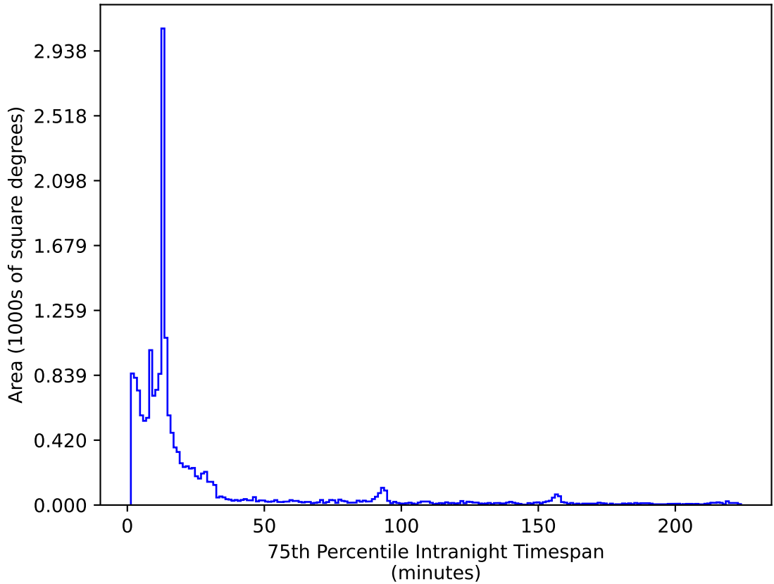
weather_cloudso18v3.4_10yrs WFD i band: 75th Percentile Intranight Timespan
