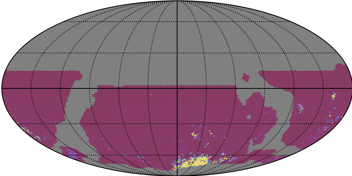
weather_cloudso18v3.4_10yrs WFD gr bands: 75th Percentile Intranight Timespan
