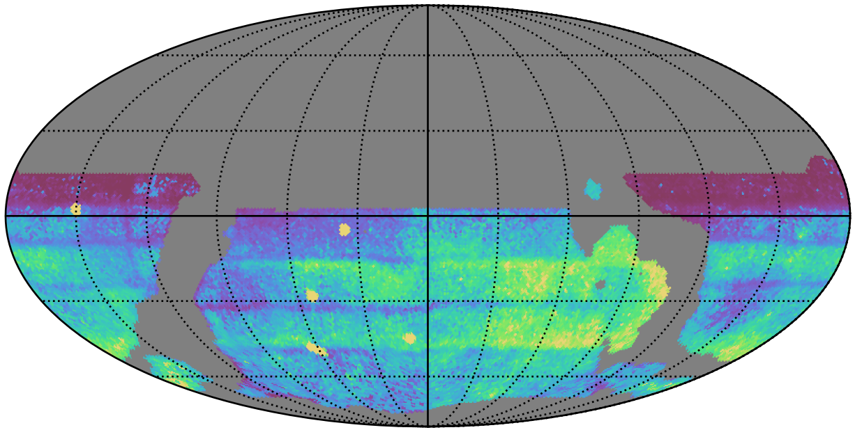
weather_cloudso18v3.4_10yrs WFD all bands: 75th Percentile Intranight Timespan
