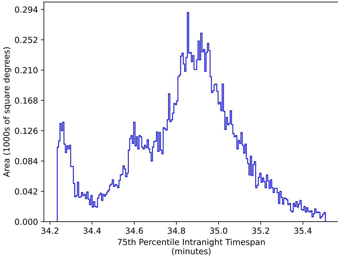
weather_cloudso18v3.4_10yrs WFD: 75th Percentile Intranight Timespan
