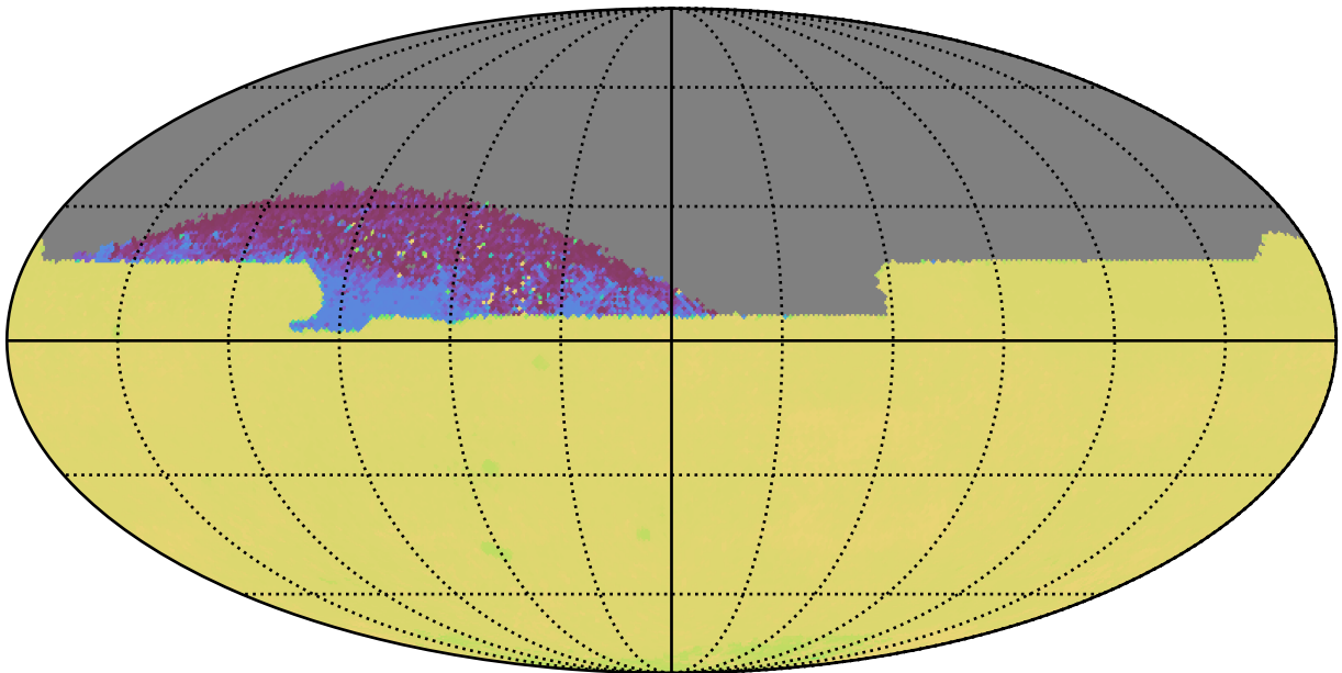
weather_cloudso18v3.4_10yrs All sky zy bands: 75th Percentile Intranight Timespan
