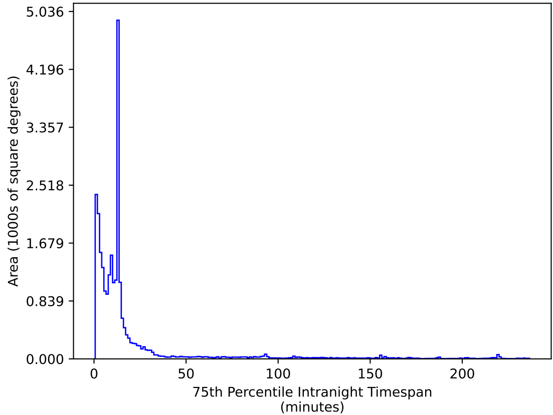
weather_cloudso18v3.4_10yrs All sky z band: 75th Percentile Intranight Timespan
