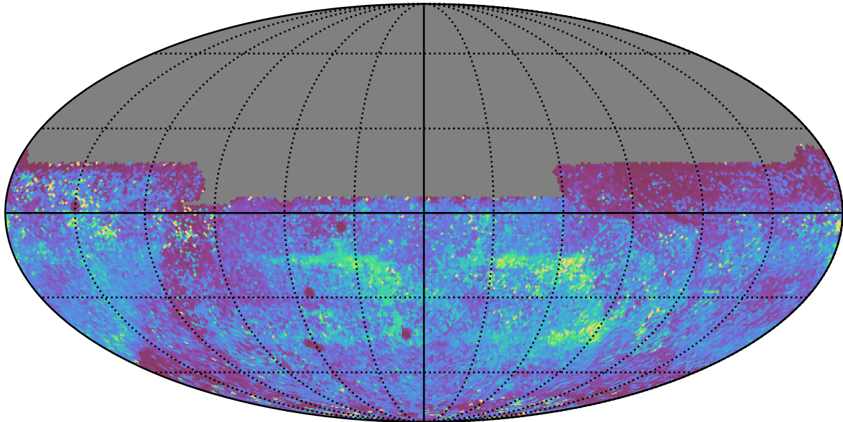
weather_cloudso18v3.4_10yrs All sky y band: 75th Percentile Intranight Timespan
