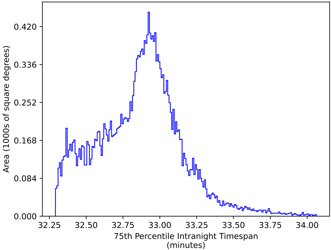
weather_cloudso18v3.4_10yrs All sky y band: 75th Percentile Intranight Timespan
