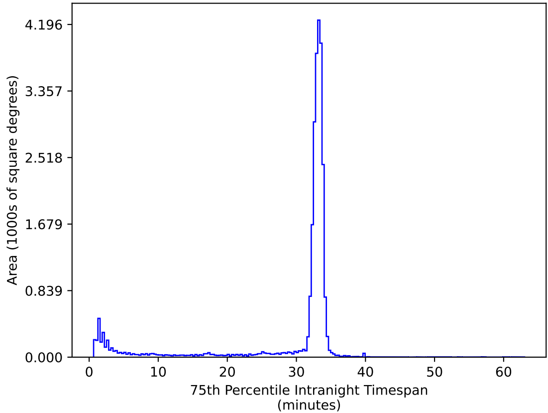
weather_cloudso18v3.4_10yrs All sky ug bands: 75th Percentile Intranight Timespan
