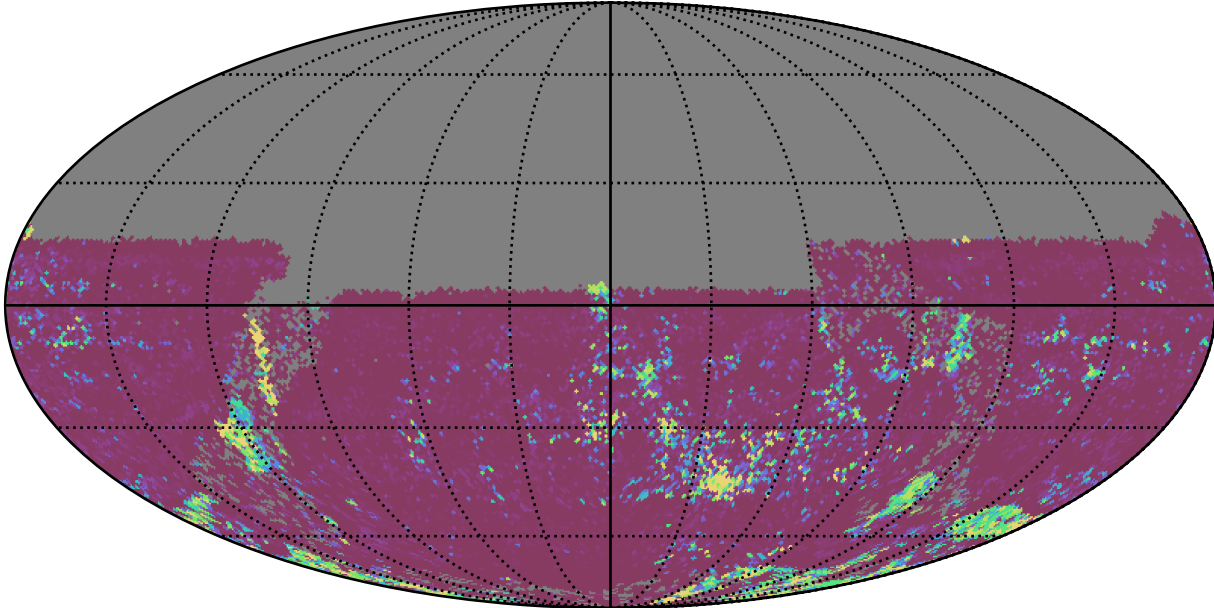
weather_cloudso18v3.4_10yrs All sky u band: 75th Percentile Intranight Timespan
